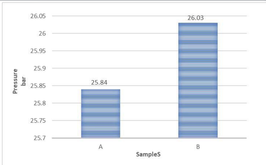
Fig (6) Average results Pressure water test of samples for types A&B
